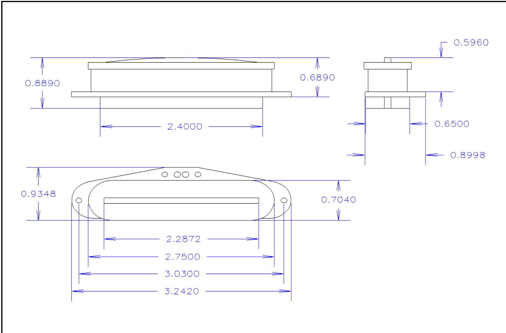
SBA single coil pickup
